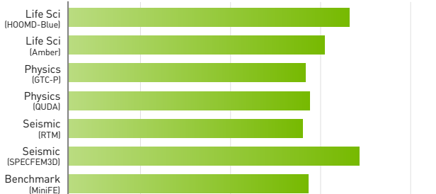
1.5X HPC Performance in One Year with NVIDIA Tesla V100
